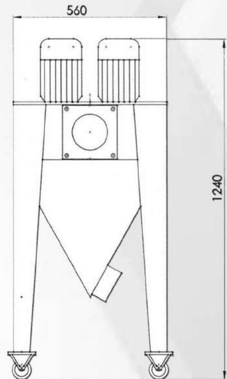
Dimensions of machine
